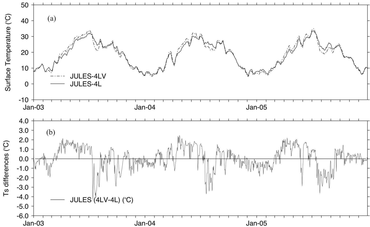
Figure 11. Modeled (a) surface temperature 10 days moving average ( ^{\circ}\text{C} ) and (b) absolute [4LV-4L] daily difference of surface temperature (in ^{\circ}\text{C} ) between modeled 4L and 4LV run for the Audubon site between 2003 and 2005.
