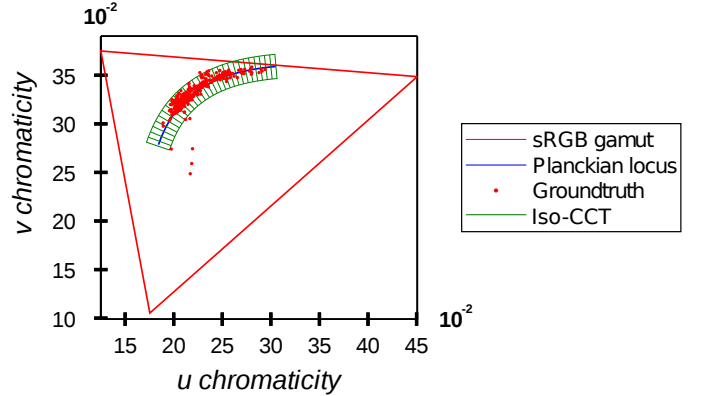
Fig. 1. Colorchecker illuminants groundtruth in the CIE 1960 uv diagram. The red triangular region represents the set of possible colors in sRGB and the blue line represents the Planckian locus (the chromaticities of the Planckian illuminants). The green region around the Planckian locus correspond to a distance threshold \delta = 0.0125 and the green lines are iso-CCT lines. Each of the 568 red points corresponds to the uv coordinates of an illuminant of the Colorchecker database. Observe that almost all the chromaticities of these illuminants lie in the chosen vicinity of the Planckian locus.
