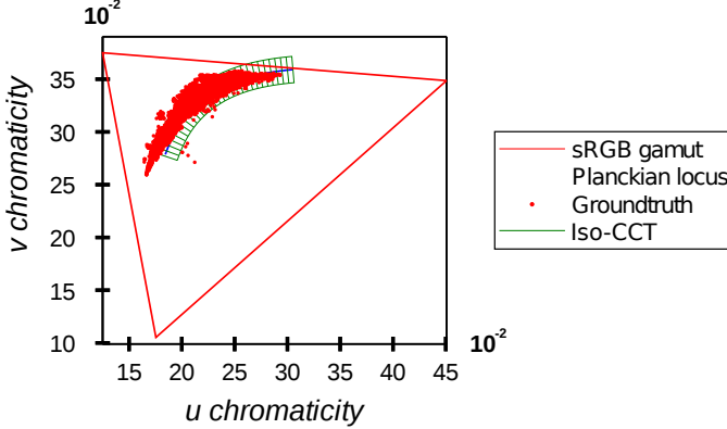
Fig. 2. Grey-Ball groundtruth illuminants projected in the CIE 1960 uv chromaticity diagram.
