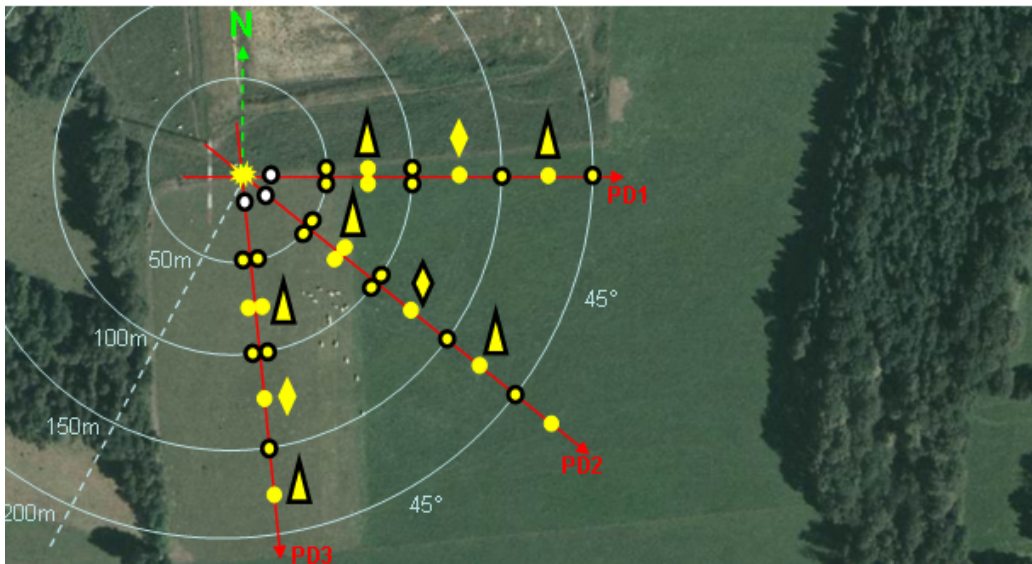
Figure 1: Lannemezan-2005 experiment, acoustical and meteorological sensor locations.
