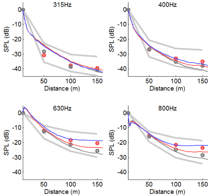
Figure 7: Sound attenuation (normalised by the free field and by a reference microphone located 10 m from the sound source) as a function of the distance from the source, for 315Hz, 400Hz, 630Hz and 800 Hz third octave bands. The bold grey lines traduce the experimental dispersion over the three-month measurements. Comparison between experimental data during the campaign of Lannemezan 2005 (points) and TLM predictions (full line) using (blue) measured meteorological conditions on 16-06-2005 at 04h30 following PD3, (grey) nearly-homogeneous conditions and (red) rough (linear) vertical profiles of sound speed.
