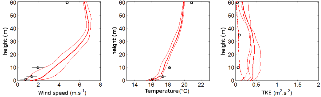
Figure 4: Mean vertical profiles (thick line) and dispersion (thin lines) of the wind speed, temperature and turbulent kinetic energy (total TKE in continuous line with dispersion, subgrid TKE in dashed line and resolved TKE in dotted line), both measured (black) and simulated (red) on 03-07-2005 at 04h30 (stable case).
