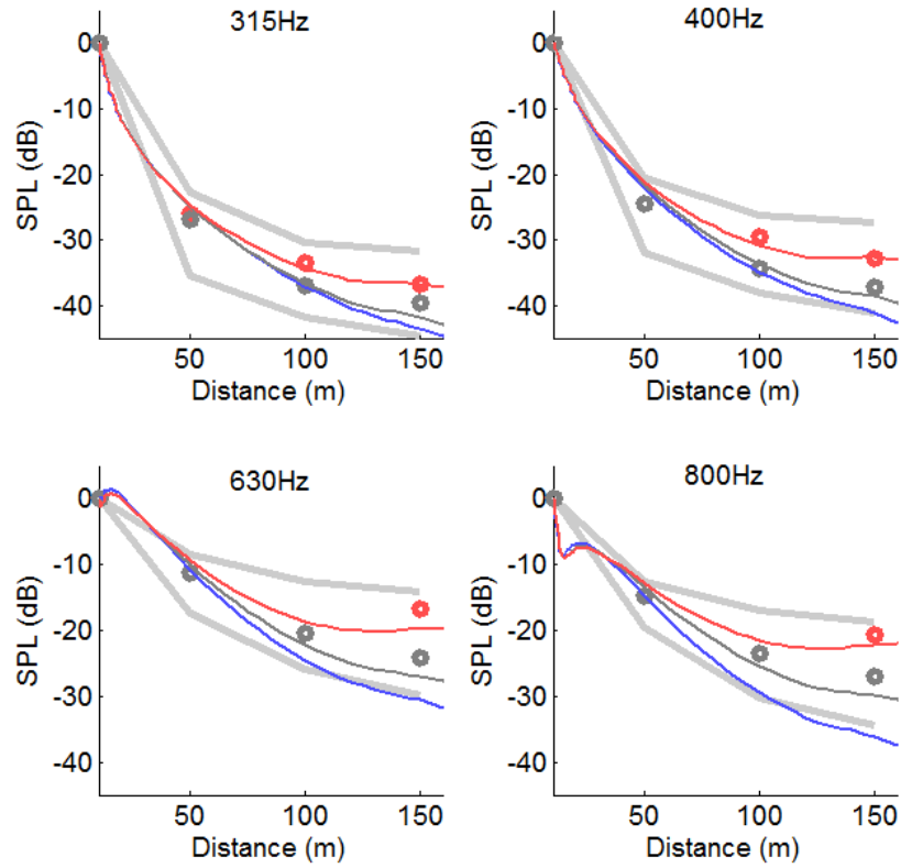
Figure 6: Sound attenuation (normalised by the free field and by a reference microphone located 10 m from the sound source) as a function of the distance from the source, for 315Hz, 400Hz, 630Hz and 800 Hz third octave bands. The bold grey lines traduce the experimental dispersion over the three-month measurements. Comparison between experimental data during the campaign of Lannemezan 2005 (points) and TLM predictions (full line) using (blue) measured meteorological conditions on 03-07-2005 at 04h30 following PD3, (grey) nearly-homogeneous conditions and (red) rough (linear) vertical profiles of sound speed.
