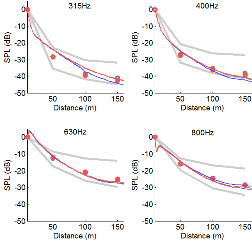
Figure 5: Sound attenuation (normalised by the free field and by a reference microphone located 10 m from the sound source) as a function of the distance from the source, for 315Hz, 400Hz, 630Hz and 800 Hz third octave bands. The bold grey lines traduce the experimental dispersion over the three-month measurements. Comparison between experimental data during the campaign of Lannemezan 2005 (points) and TLM predictions (full line) using (blue) measured meteorological conditions on 17-06-2005 at 16h30 following PD3, (grey) nearly-homogeneous conditions and (red) rough (linear) vertical profiles of sound speed.
