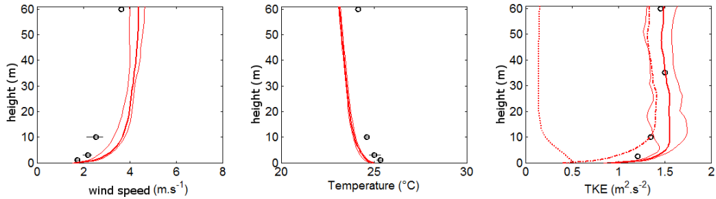
Figure 3: Mean vertical profiles (thick line) and dispersion (thin lines) of the wind speed, temperature and turbulent kinetic energy (total TKE in continuous line with dispersion, subgrid TKE in dashed line and resolved TKE in dotted line), both measured (black) and simulated (red) on 17-06-2005 at 16h30 (unstable case).
