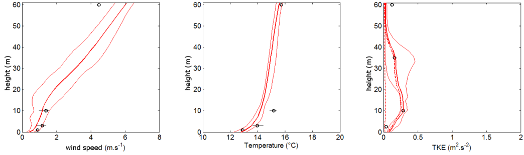
Figure 2: Mean vertical profiles (thick line) and dispersion (thin lines) of the wind speed, temperature and turbulent kinetic energy (total TKE in continuous line with dispersion, subgrid TKE in dashed line and resolved TKE in dotted line), both measured (black) and simulated (red) on 16-06-2005 at 04h30 (neutral case).
