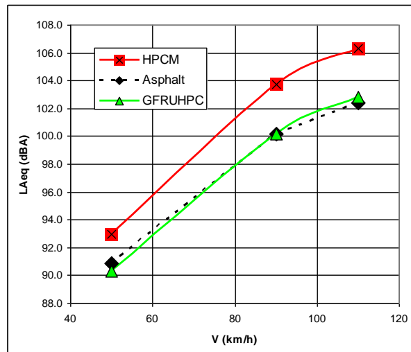
Figure 7 : noise generation as measured by the CPX method on the Loire-Atlantique test section (3rd track), after two weeks of traffic.
