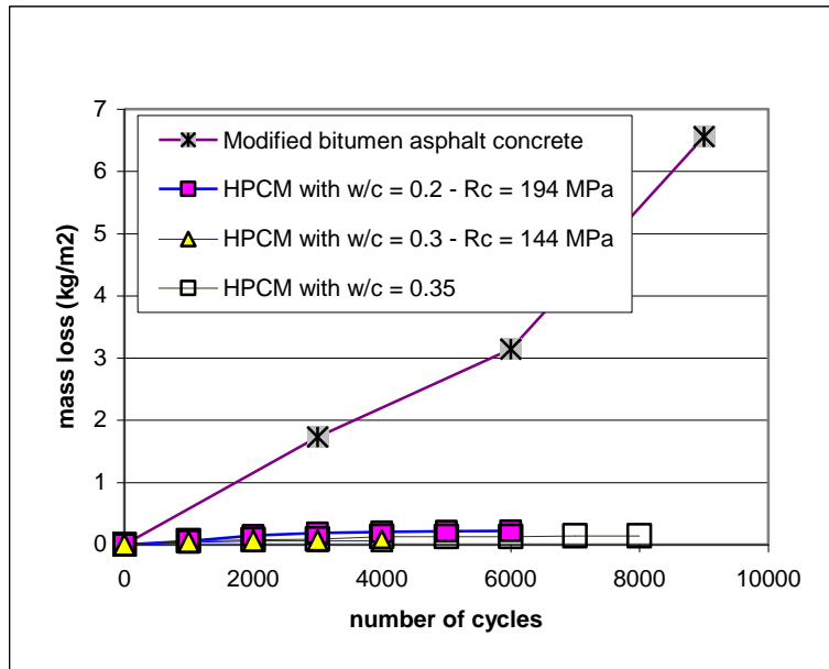
Figure 3 : resistance to wear of HPCM, compared to that of modified bitumen asphalt, as measured with the Triboroute™ apparatus. No loss of material is found for hydraulic solutions.
