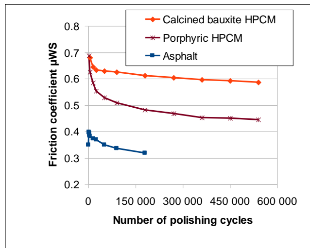
Figure 4 : skid-resistance of HPCM, as measured with the Shulze machine [7].
