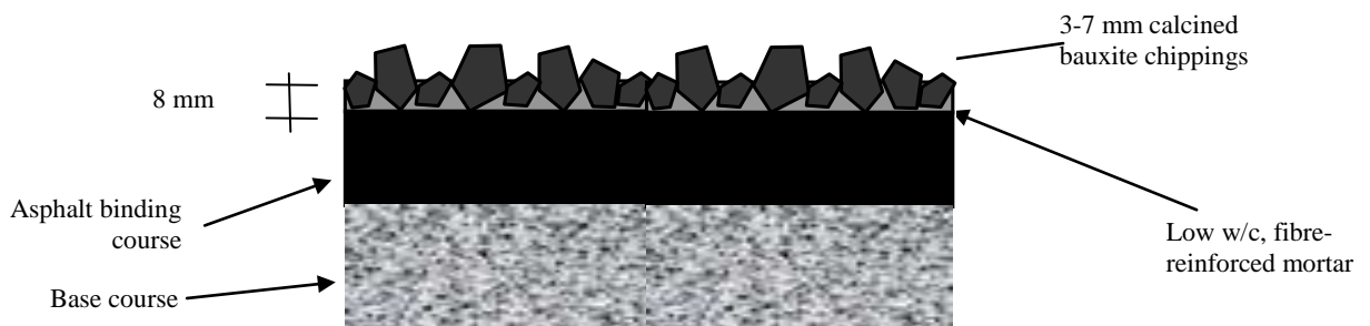
Figure 1 : principle of the High-Performance Cementitious Material (HPCM) [2].
