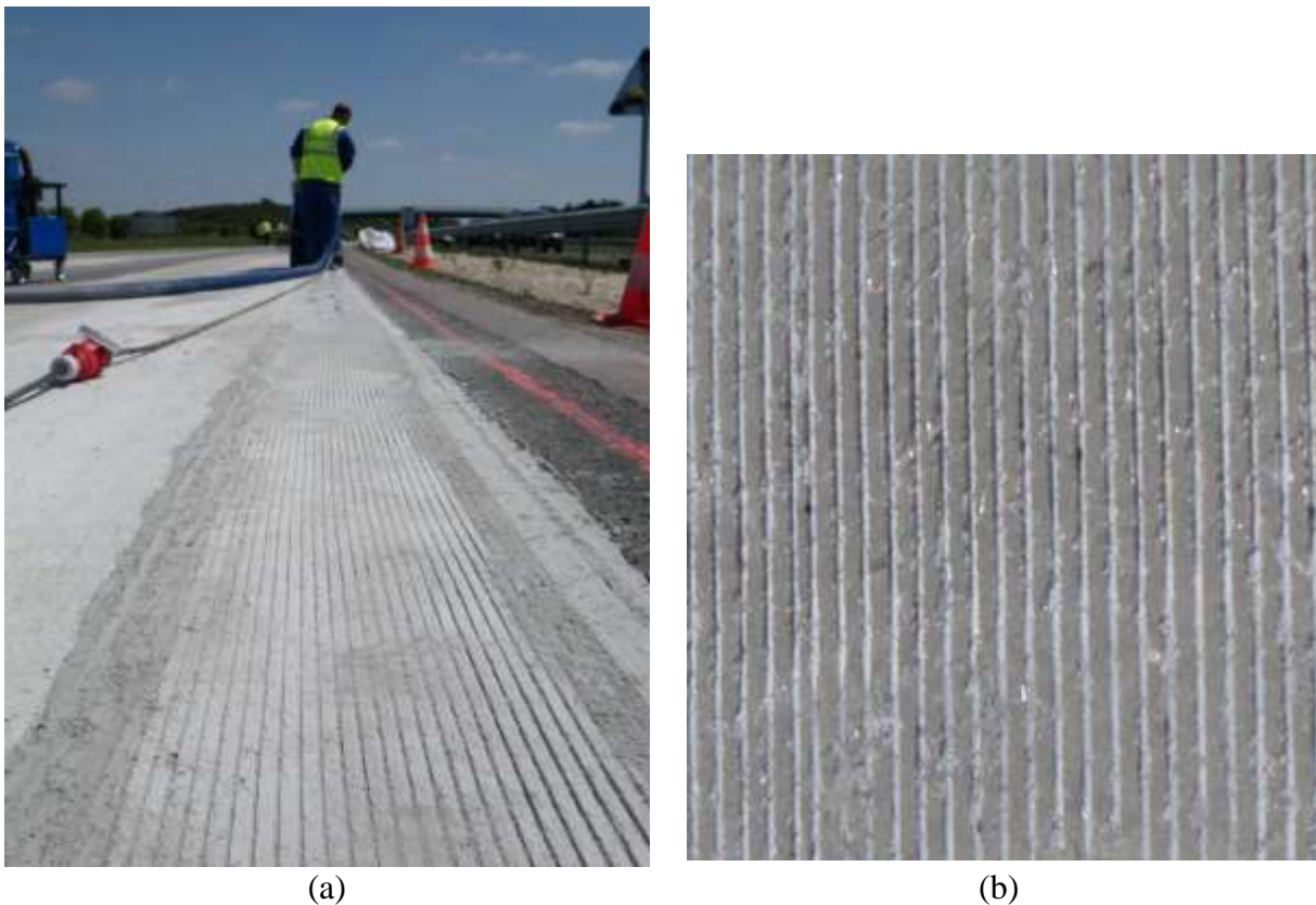
Figure 5 : Grooved Fibre-Reinforced Ultra-High Performance Concrete, as applied on the second CLEAN construction site.(a) : grooving with a diamond saw. (b) : final aspect. Grooving spec. : inter-axle distance 10 mm, width 4.5 mm, depth 3 mm.
