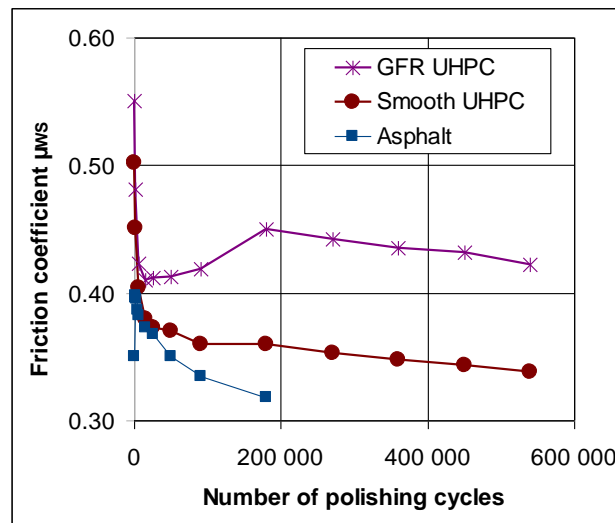
Figure 6 : skid-resistance of GFR UHPC, as measured with the Wehner & Shulze machine.
