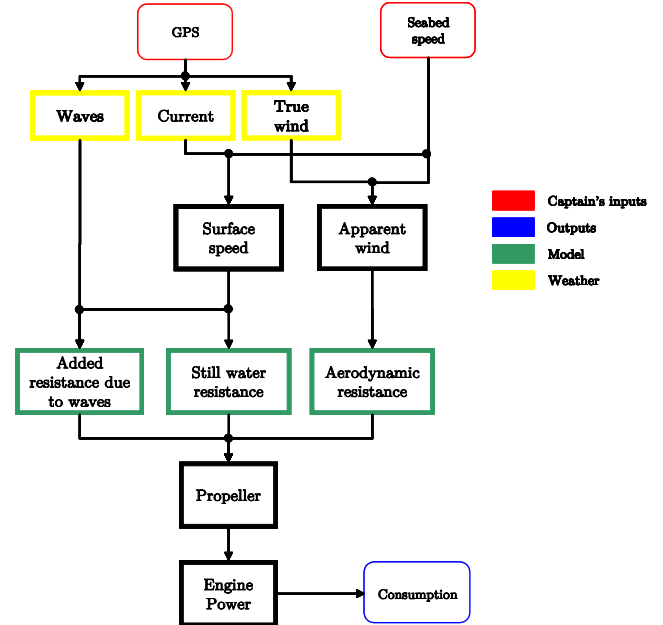
Figure 5: Scheme calculation of the consumption
