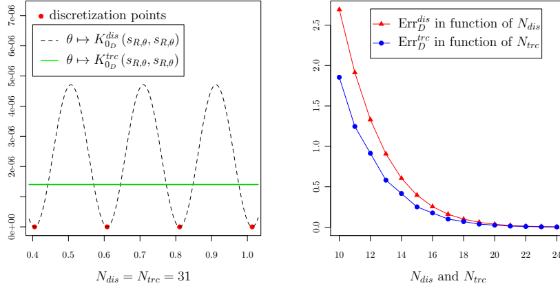
FIGURE 5. Graphs of \theta \mapsto K_{0D}^{trc}(s_{R,\theta}, s_{R,\theta}) and \theta \mapsto K_{0D}^{dis}(s_{R,\theta}, s_{R,\theta}) (with \theta \in [0, 2\pi) ) for N_{trc} = N_{dis} = 31 (left) and values of the terms \text{Err}_D^{dis} and \text{Err}_D^{trc} for 10 \leq N_{dis}, N_{trc} \leq 24 (right) with R = 3 and \sigma^2 = 2 .
