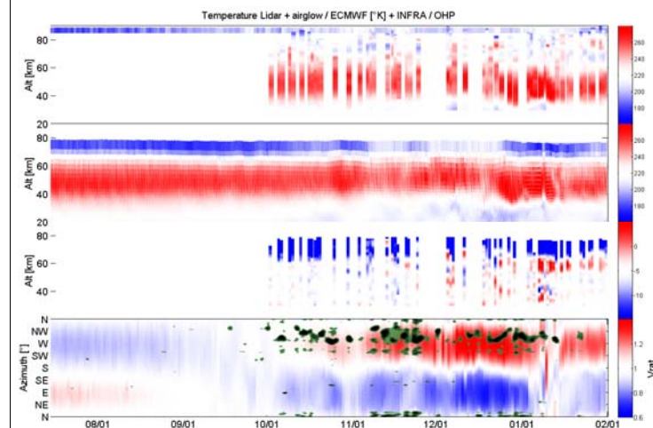
Figure 4 - Multi-technology synthetic view at Haute-Provence Observatory. From top to bottom: Lidar measurements, ECMWF temperature model, difference between Lidar and ECMWF, logarithm of the number of microbarom detections superimposed to the effective sound-speed ratio (ECMWF).
