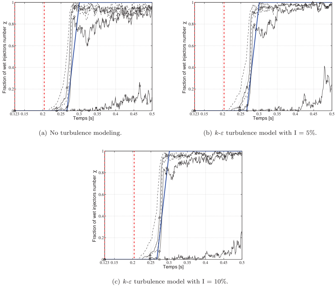
Figure 14: Influence of the turbulence modeling on the evolution of the fraction of wet injectors number \chi . — : Experimental wet law, ---- : Threshold 0.0001%, ..... : Threshold 0.01%, —△— : Threshold 0.1%, -.-.- : Threshold 1%, —○— : Threshold 10%, —□— : Threshold 100%, - - - - : valve position.
