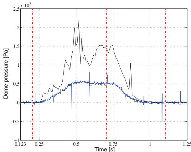
Figure 9: Comparison of the dome pressure. \text{---}\square\text{---} : Experimental pressure, \text{---} : numerical pressure, \text{-}\cdot\text{-}\cdot\text{-}\cdot\text{-} : valve position.
