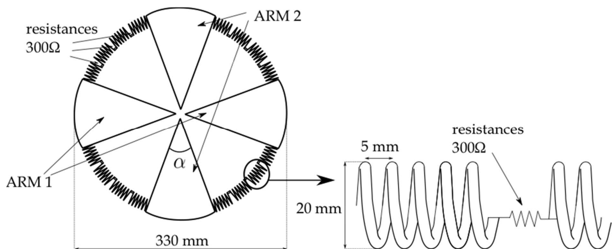
Fig. 1 - Antenna design and dimensions of the coil.
