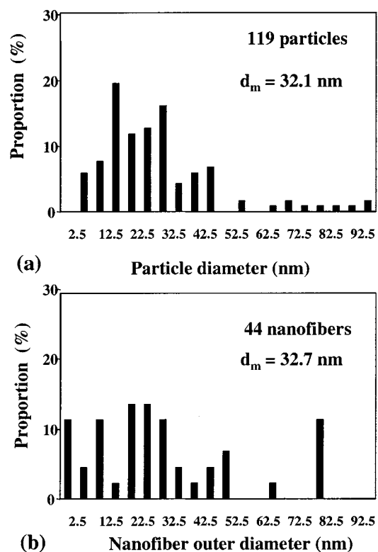
Figure 7. Particle-size (a) and nanofiber outer-diameter (b) distributions in Fe10U1R evaluated from TEM images (similar to those shown in Figure 3). Each class noted by a value of x nm corresponds to particle sizes or nanofiber outer diameters contained between (x - 2.5 nm) and (x + 2.5 nm). For both distributions, the number of measurements and the average value ( d_m and d_{om} ) are indicated.
