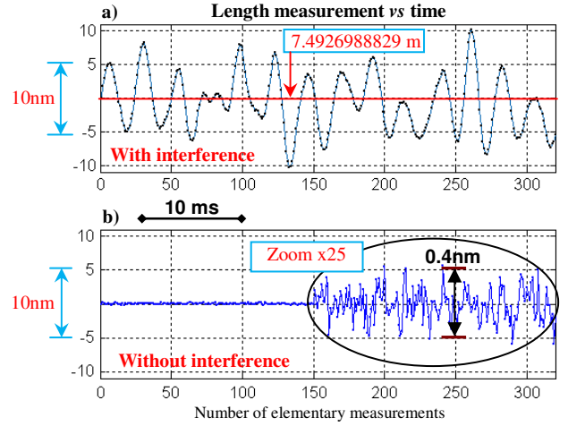
Figure 12. Results of 320 elementary cycles in 43 ms.
