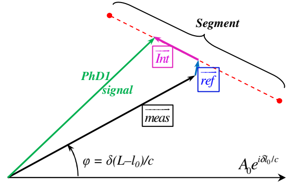
Figure 2. Addition, in the complex plane, of the three contributions to the PhD1 two-mode interference, signal. The phase e^{i\delta l_0/c} , of the PhD0 photodiode, is taken as the phase reference.
