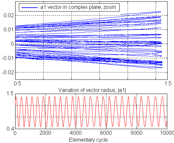
Figure 15. The "spikes" of the telemetric signal trajectory in the complex plane when the measurement path length is varied by 25\lambda_{\text{opt}} \approx 39 \mu\text{m} in 10 mn
