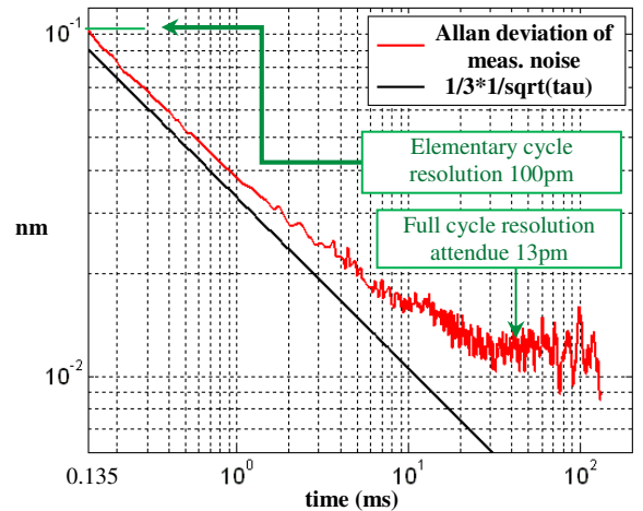
Figure 13. The expected resolution of the telemetric measurement. Same data as in Fig. 12 b)
