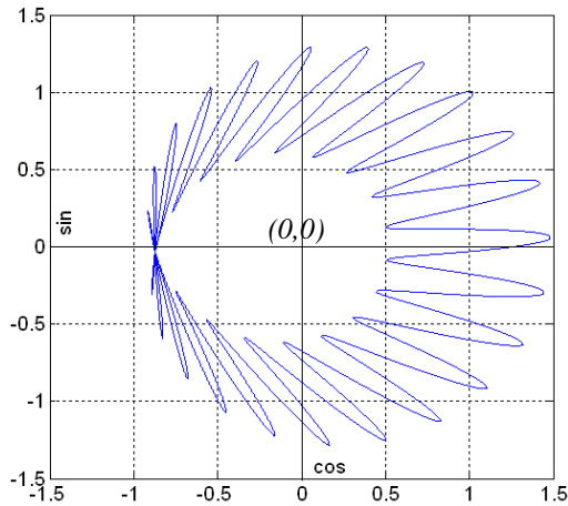
Figure 3. The calculated two-mode interference pattern obtained, at constant \nu_{opt} , when the target is moved continuously over \Lambda/2 , with \varepsilon = 0.25
