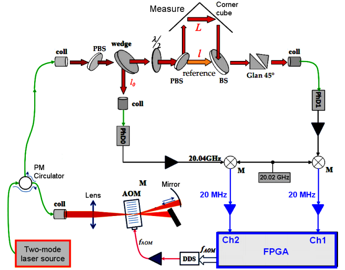
Figure 5. Experimental setup
