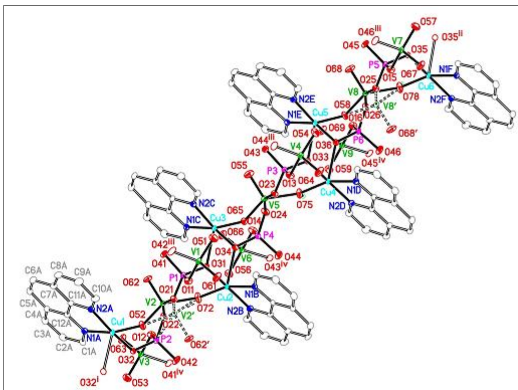
Figure 1. Molecular view of 1a with displacement ellipsoids at a 30% level. Carbon atoms in the phenyl ligands "B" to "F" are not labelled in the Figure, but repeat the labelling scheme as those in the "A" moiety. Aromatic H atoms omitted. Symmetry codes: (i) -x+2, -y, -z ; (ii) -x, -y+2, -z+1 ; (iii) x-1, y, z ; (iv) x+1, y, z .
