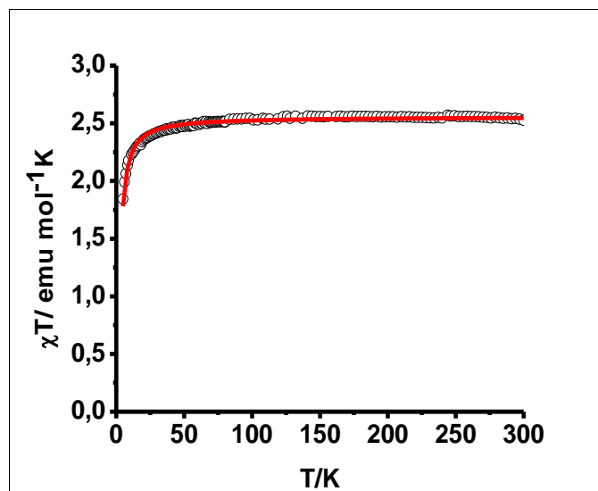
Figure 4. Temperature dependence of \chi T for 1a . Open circles represent the experimental magnetic susceptibility data; red line corresponds to the fit using the van Vleck analytical expression.
