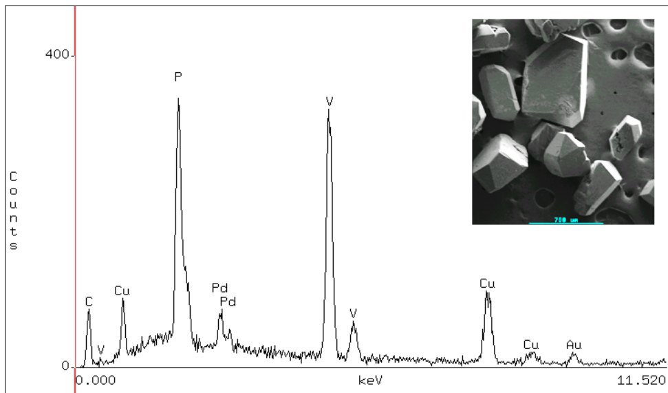
Figure 1S. Spectrum SEM-EDXS of 1a .
