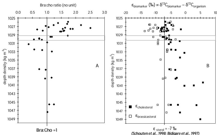
Fig. 5. Panel A = vertical profile of small particle brassicasterol vs. cholesterol concentrations ratio (no unit; from Table 2) for the whole dataset. Panel B = vertical profile of \epsilon_{\text{cholesterol}} and \epsilon_{\text{brassicasterol}} for the whole dataset ( \epsilon_{\text{sterol}} (\text{‰}) = \delta^{13}\text{C}_{\text{sterol}} - \delta^{13}\text{C}_{\text{SP-POC}} ). The grey rectangle represents the range of 500 m depth horizons along the transect (see Table 2).
