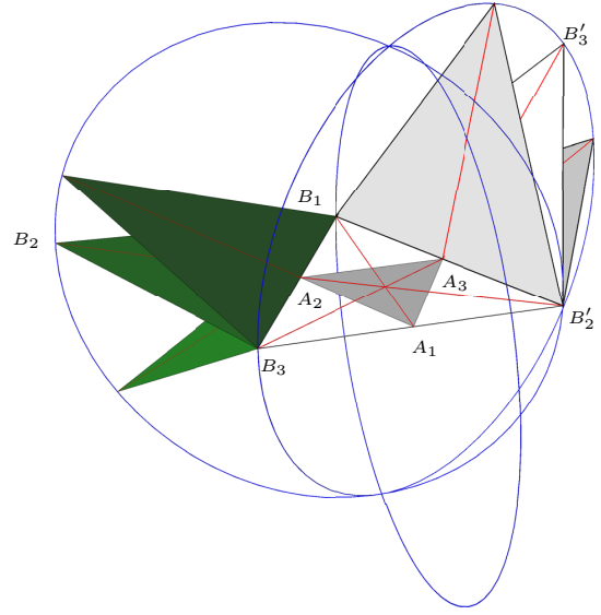
Figure 3: Special case h_2 = 2
