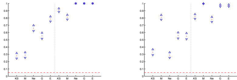
Figure 2: Left: (s_1, s_2) = (f_1, f_{4,\varepsilon}) . The two columns resp. correspond to \varepsilon = 0.5 and 1 . Right: (s_1, s_2) = (f_{5,\lambda}, f_{6,1/2,1/4}) . The two columns resp. correspond to \lambda = 7 and \lambda = 10 .
