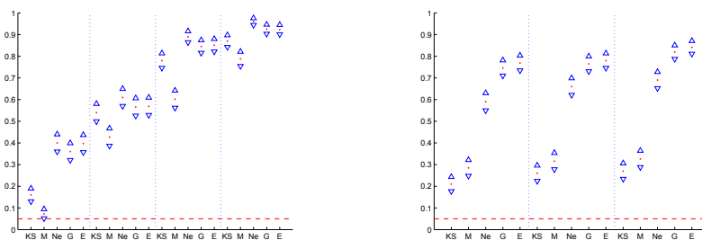
Figure 1: Left: (s_1, s_2) = (f_1, f_{2,a,\varepsilon}) . Each column resp. corresponds to (a, \varepsilon) = (1/8, 1), (1/4, 0.7), (1/4, 0.9), and (1/4, 1) . Right: (s_1, s_2) = (f_1, f_{3,\eta}) . Each column resp. corresponds to \eta = 4, 8 and 15 .
