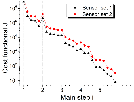
FIGURE 7 – Cost functional evolution through iterations in both i and j loops and for both sensors sets
