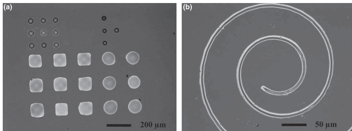
Fig. 2. Examples of micrometric features of catalyst precursor made by \mu\text{CP} : (a) 105 and 55 \mu\text{m} large patterns (squares or dots); (b) 10 \mu\text{m} wide spiral.
