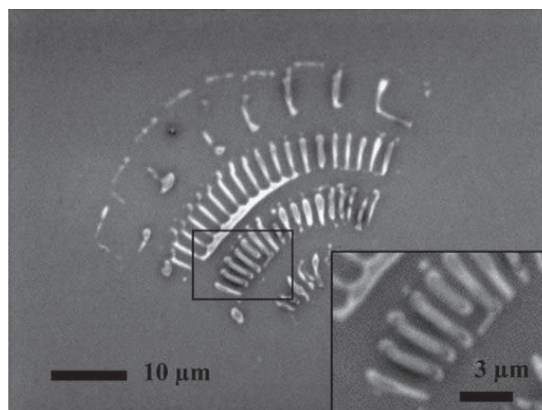
Fig. 3. Catalyst precursor features deposited by \mu\text{CP} . The softness of our stamp limits the fidelity of the printed features to those of the stamp.
