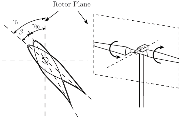
Fig. 8: Schematic of a blade with pitch control
