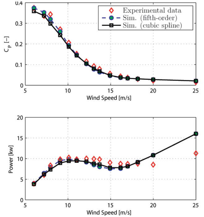
Fig. 6: Comparison between simulated and experimental results
