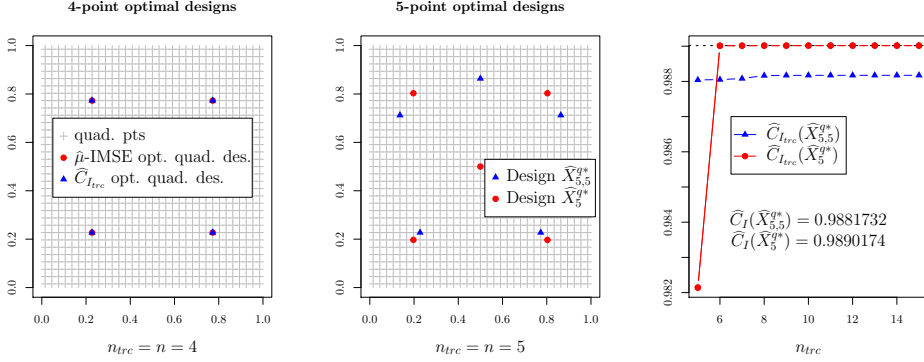
FIGURE 5.4. Quadrature-designs optimal for the criteria \hat{C}_I and \hat{C}_{I_{trc}} for n = n_{trc} = 4 (left) and n = n_{trc} = 5 (middle). Values of the criterion \hat{C}_{I_{trc}} for the two quadrature-designs \hat{X}_{5,5}^{q*} and \hat{X}_5^{q*} (respectively optimal for \hat{C}_I and \hat{C}_{I_{trc}} with n_{trc} = 5 ) as functions of n_{trc} (right).
