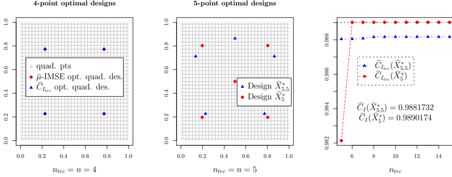
FIGURE 5.5. Quadrature designs optimal for the criteria \widehat{C}_I and \widehat{C}_{I_{trc}} for n = n_{trc} = 4 (left) and n = n_{trc} = 5 (middle). Values of the criterion \widehat{C}_{I_{trc}} for the two quadrature designs \widehat{X}_5^* and \widehat{X}_{5,5}^* (respectively optimal for \widehat{C}_I and \widehat{C}_{I_{trc}} with n_{trc} = 5 ) as function of the number n_{trc} of considered eigenvalues (right).
