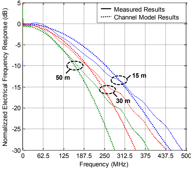
Fig. 3. Normalized frequency responses of SI-POF with different length parameters in TABLE I.
