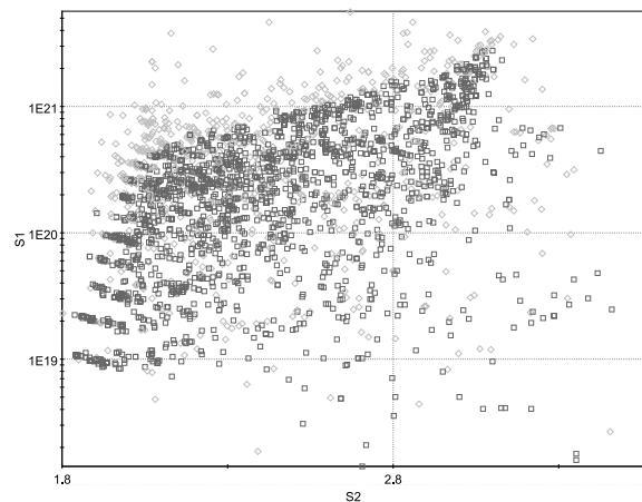
Fig. 8. Scatter chart of S_1 versus S_2 .
