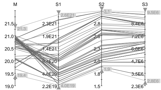
Fig. 9. Parallel coordinates chart of the Pareto-optimal designs.
