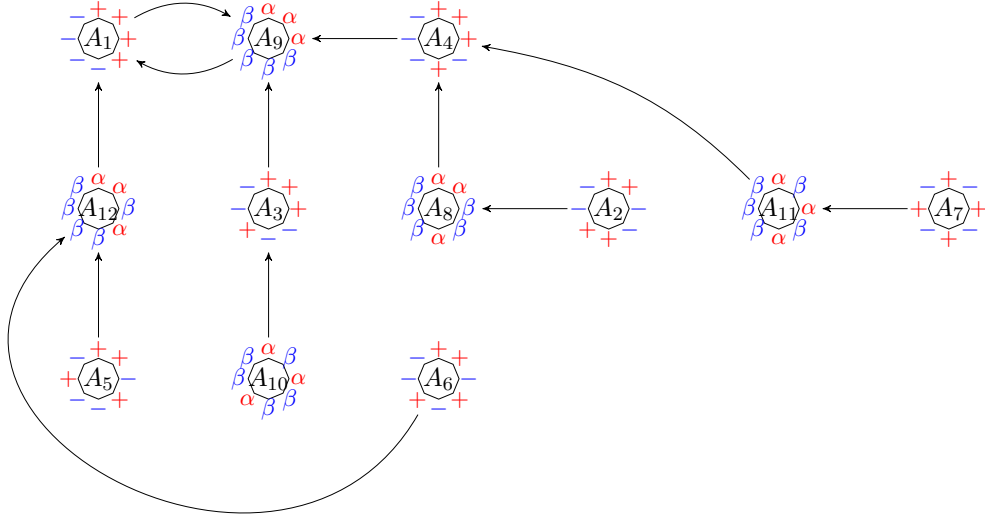
FIGURE 8. The graph of successors for N = 8 .
