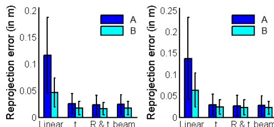
Fig. 6. Mean and standard deviation of reprojection error. Computed with orthogonal distance (left) and beam metric (right) for the chessboard plane data set (A) and the modified chessboard plane data set (B)
