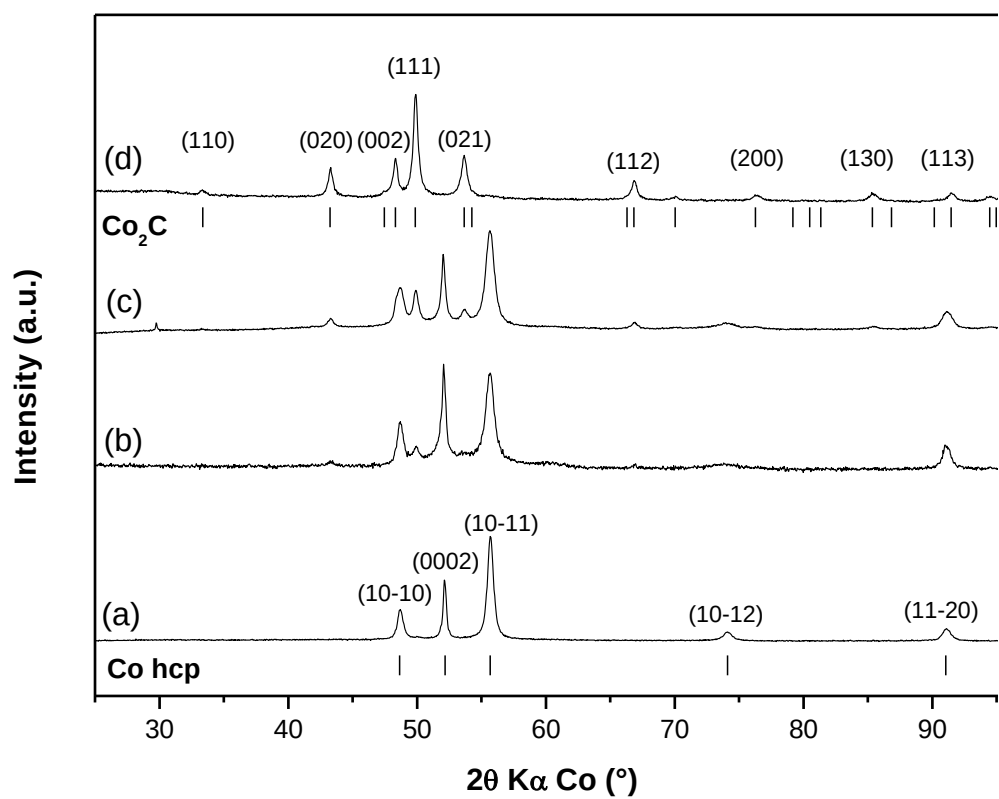
Figure 4 XRD pattern of Co rods treated (a) in ODE for 3h and in a mixture of ODE/OA for (b) 30 min, (c) 3h and (d) 4h (only the \text{Co}_2\text{C} strongest lines are indexed).
