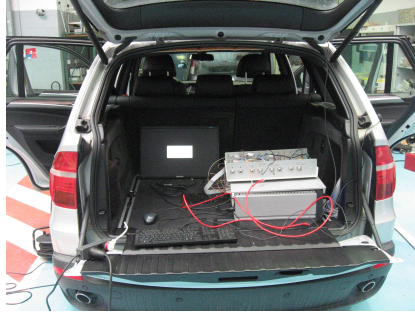
(a) Integration of the SDR platform on a BMW X5 test vehicle
