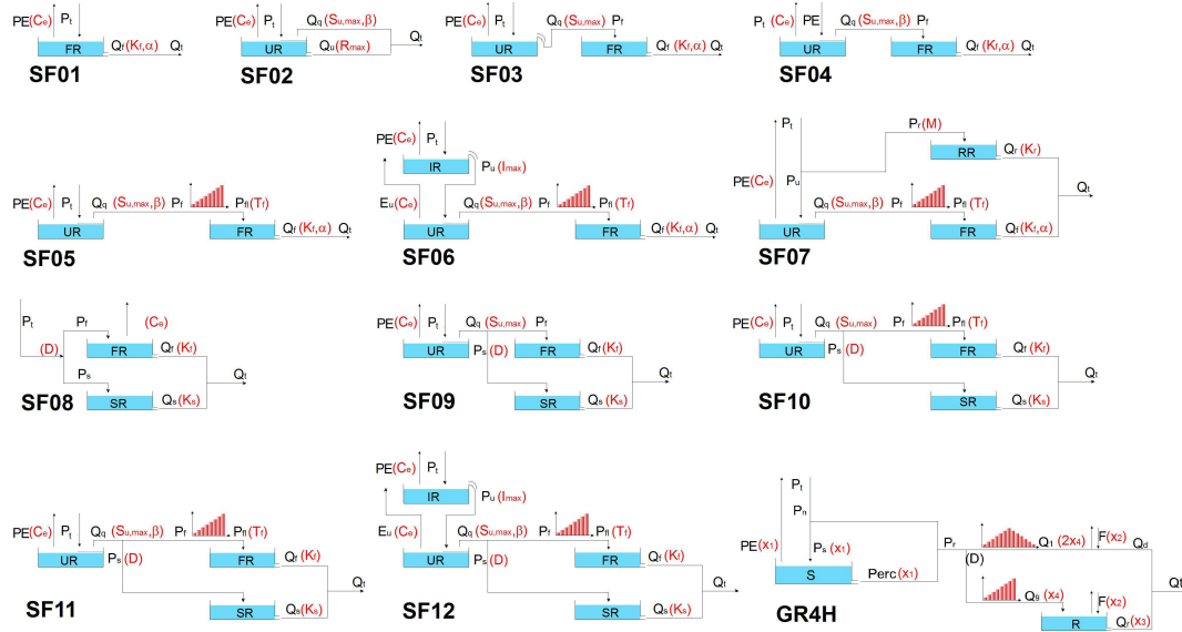
Fig. 2. Schematics of the 12 model structures generated using the SUPERFLEX framework (SF01–SF12 by Fenicia et al., 2013) and the GR4H model (Perrin et al., 2003). A flux of water is denoted in black next to an arrow line. Parameters are given in brackets in red font.
