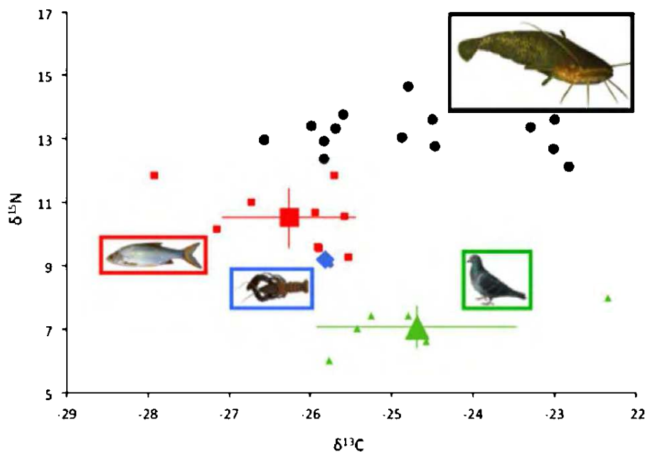
Figure 2. Stable isotope values of European catfish and the putative prey. \delta^{13}\text{C} and \delta^{15}\text{N} values (‰) of each individual ( n=14 ) and the putative aquatic (fish, n=9 and crayfish, n=3 ) and terrestrial (pigeon, n=6 ) prey are displayed. The large symbols for each prey represent the mean value ( \pm SD).
