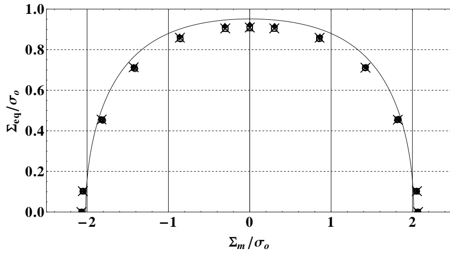
Figure 8: Spherical intergranular voids, von Mises matrix, Lode angle \omega = \pi/6 , drained conditions ( p_b = p_e = 0 ). Solid line: Gurson criterion with porosity q \times 0.04 , q = 1.214 . Symbols: FFT results for the 6 microstructures of Figure 6 all 6 symbols are almost on top of each other).
