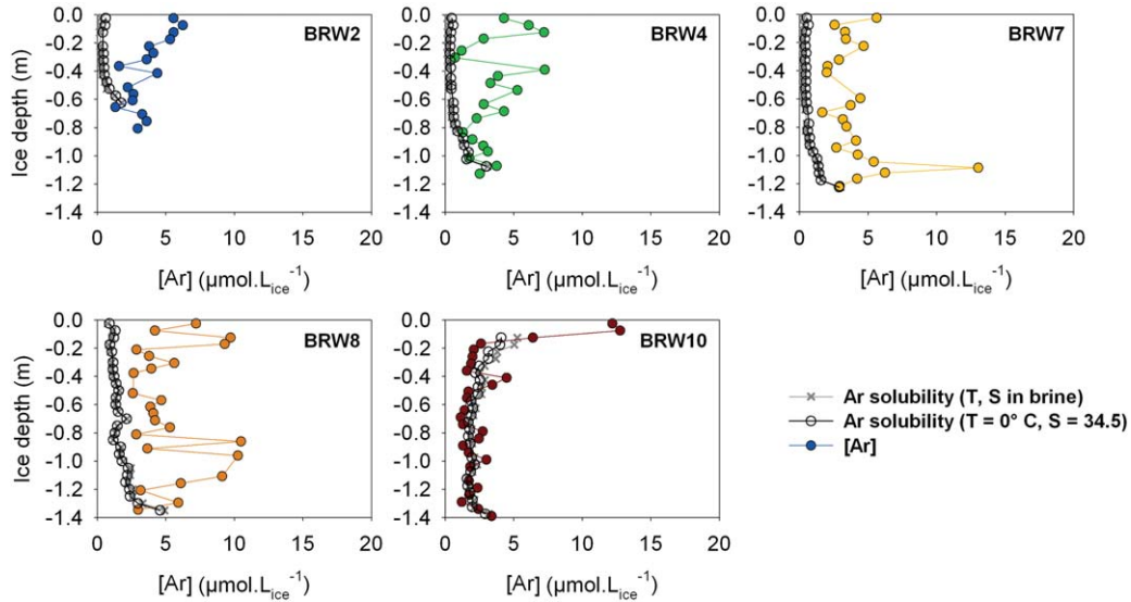
Figure 11. Evolution of Ar concentration ( [Ar] ) in bulk sea ice (dots) as compared to the solubility limits in sea ice calculated using temperature and salinity in brine (crosses) or temperature and salinity fixed at 0^{\circ}\text{C} and 34.5, respectively (empty dots). Deviation of [Ar] in bulk ice to the solubility limit indicates potential bubble content, while [Ar] in bulk ice at the solubility limit indicates that the gas is dissolved in brine.
