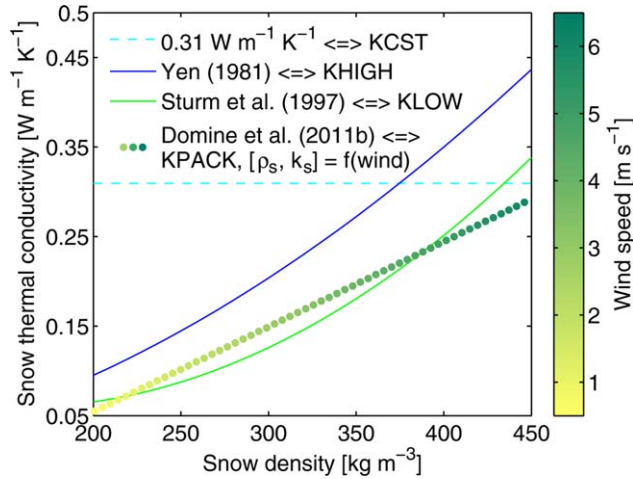
Figure 2. Snow thermal conductivity versus density for Yen [1981] and Sturm et al. [1997] relationships. Colored dots of coordinates (\rho_s, k_s) represent snow thermal conductivity and density as functions of wind speed from Domine et al. [2011b].
