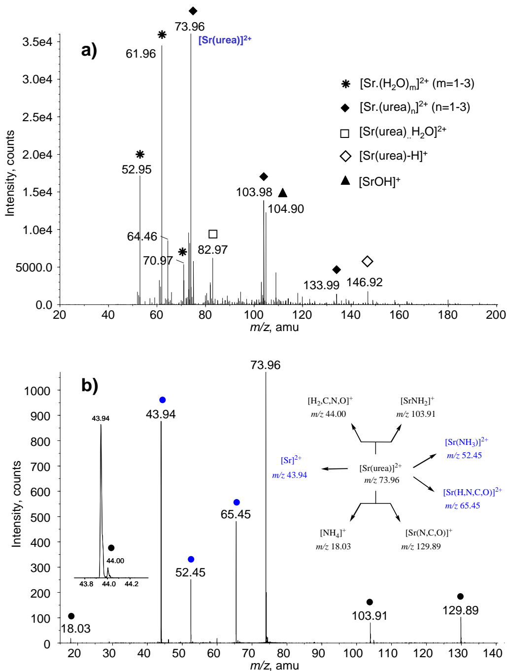
Figure 1: a) Positive-ion electrospray spectrum of an equimolar aqueous \text{SrCl}_2/\text{urea} ( 10^{-4} mol \text{L}^{-1} ) mixture, recorded with a declustering potential of 40 V; b) Low-energy CID spectrum of the [\text{Sr}(\text{urea})]^{2+} complex recorded with a collision energy of 13 eV (laboratory frame) See text for details
