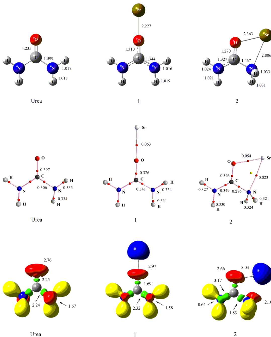
Figure 2. Optimized structures, molecular graphs and ELF plots for urea and the most stable urea- \text{Sr}^{2+} adducts. Bond lengths are in Å. The densities at the BCPs (red dots) in the molecular graphs are in a.u.. In the ELF plots, blue, red, green basins correspond to core-pairs, lone-pairs, bonding pairs, respectively. Yellow basins denote disynaptic basins associated with XH bonds. Electron populations are in e.
