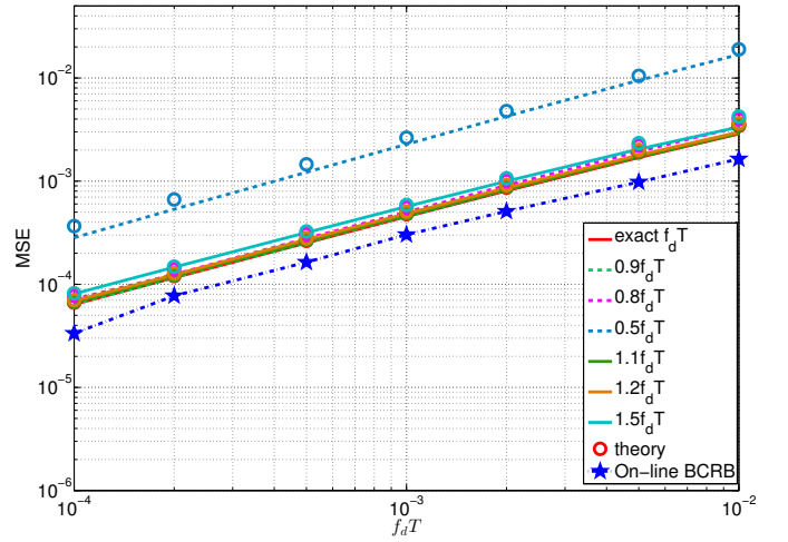
Fig. 8: Effect of a mismatch on the knowledge of f_d : MSE versus f_d T , f_d T' (used to tune the RW3-CATL) shifted 10%, 20%, 50% from the true value and \text{SNR} = 20 dB
