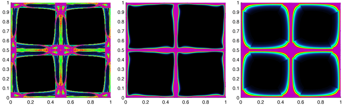
Figure 9: Taylor Green Vortices for St=St_c : number density field at time t=4 for the Lagrangian tracking (left), for the Eulerian Isotropic Gaussian closure (center), and for the Eulerian Anisotropic Gaussian closure (right).
