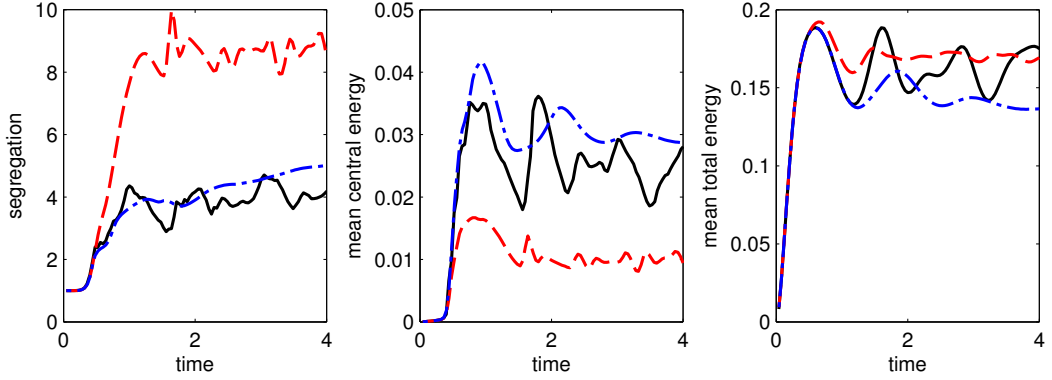
Figure 13: Taylor Green Vortices for St=5St_c : time evolution of the segregation (left), mean central energy (center), and mean total energy (right) for the Lagrangian tracking (black full line), the Eulerian Isotropic (red dashed line) and Anisotropic (blue dot-dashed line) Gaussian closures.
