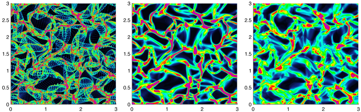
Figure 16: HIT case for St = 10 : number density field at time t = 3.6 for the Lagrangian tracking (left), for the Eulerian Isotropic Gaussian closure (center), and for the Eulerian Anisotropic Gaussian closure (right).
