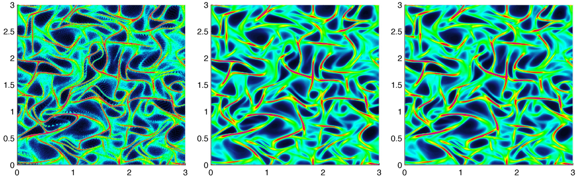
Figure 15: HIT case for St = 1 : number density field at time t = 3.6 for the Lagrangian tracking (left), for the Eulerian Isotropic Gaussian closure (center), and for the Eulerian Anisotropic Gaussian closure (right).
