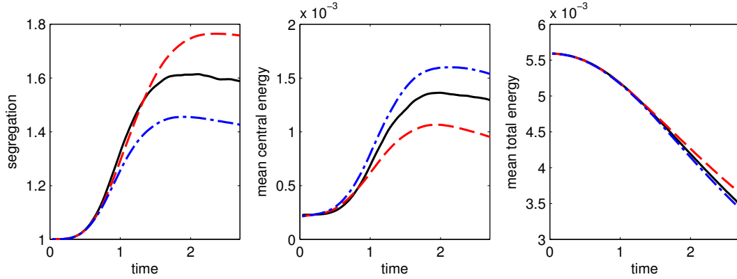
Figure 18: HIT case for St = 10 : time evolution of the segregation (left), mean central energy (center), and mean total energy (right) for the Lagrangian tracking (black full line), the Eulerian Isotropic (red dashed line) and Anisotropic (blue dot-dashed line) Gaussian closures.
