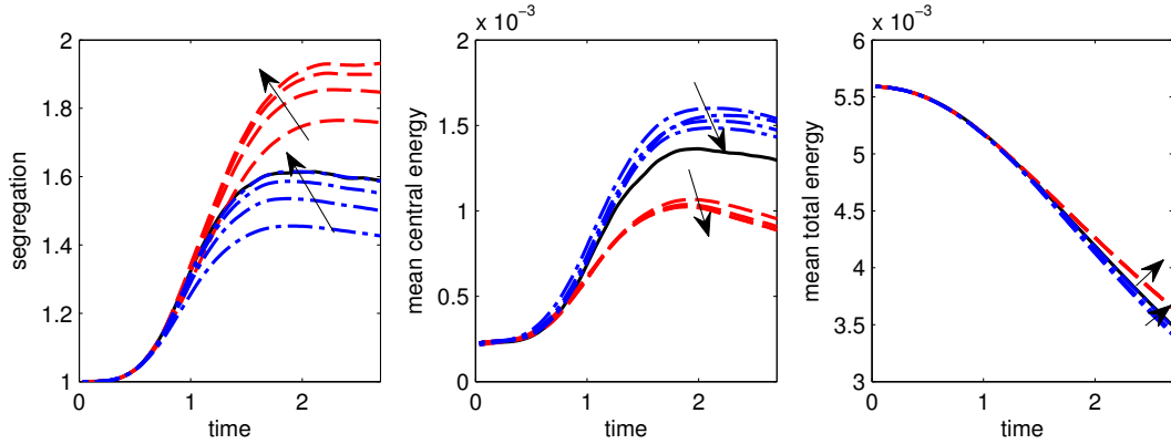
Figure 19: HIT case for St = 10 , impact of the mesh on statistics: time evolution of the segregation (left), mean central energy (center), and mean total energy (right) for the Lagrangian tracking (black full line), the Eulerian Isotropic (red dashed line) and Anisotropic (blue dot-dashed line) Gaussian closures. Arrows indicates growing meshes for each Eulerian model (from 256^2 to 2048^2 cells).
