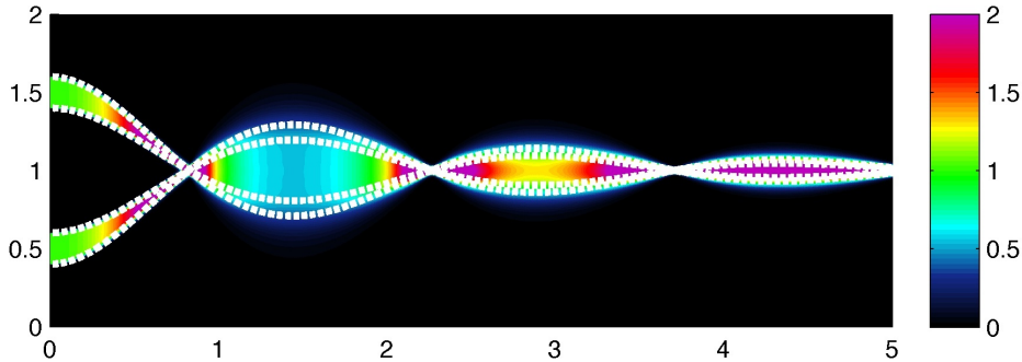
Figure 5: Steady solution of two inertial particle jets ( St=20 ) injected in a compressive velocity field: Particle number density ( m^{-3} ). White lines represent the lower and upper Lagrangian trajectories for each jet.
