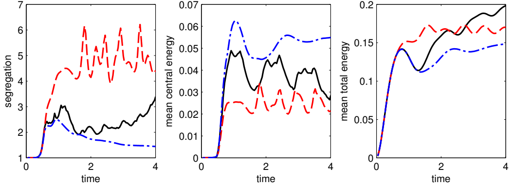
Figure 14: Taylor Green Vortices for St=10St_c : time evolution of the segregation (left), mean central energy (center), and mean total energy (right) for the Lagrangian tracking (black full line), the Eulerian Isotropic (red dashed line) and Anisotropic (blue dot-dashed line) Gaussian closures.
