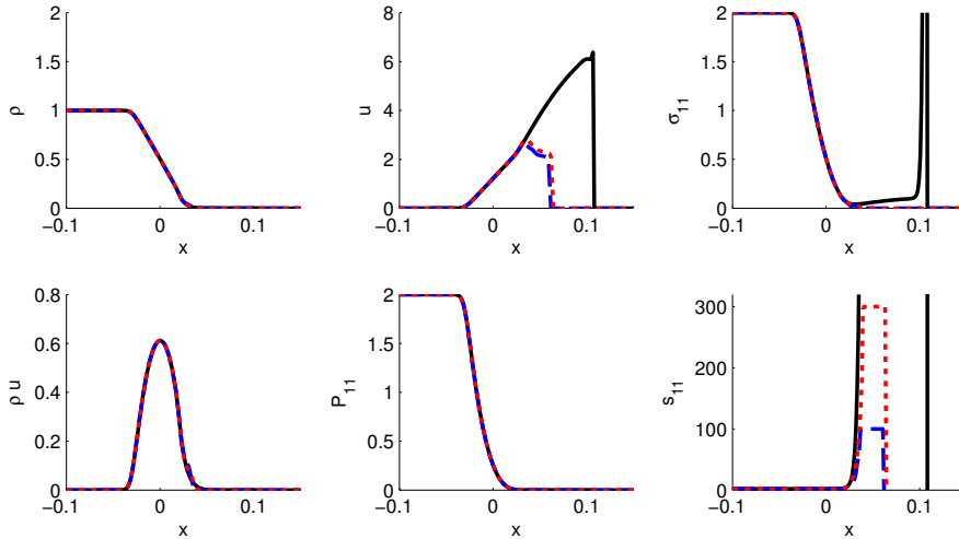
Figure 4: Riemann problem with vacuum at time t=0.05 s: MUSCL/HLL scheme with 200 cells without limitation (black full line), with S_{max}=100 (blue dashed line) and with S_{max}=300 (red dotted line).
