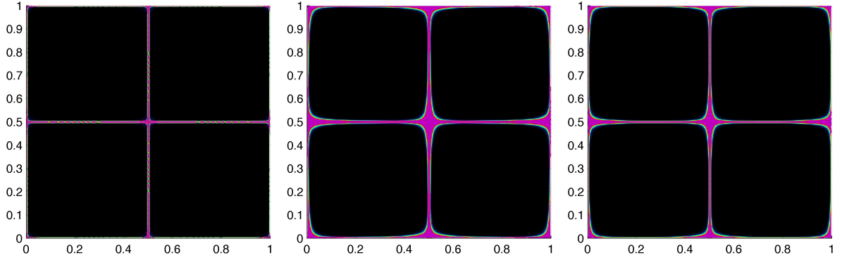
Figure 9: Taylor Green Vortices for St=St_c : number density field at time t=4 for the Lagrangian tracking (left), for the Eulerian Isotropic Gaussian closure (center), and for the Eulerian Anisotropic Gaussian closure (right).
