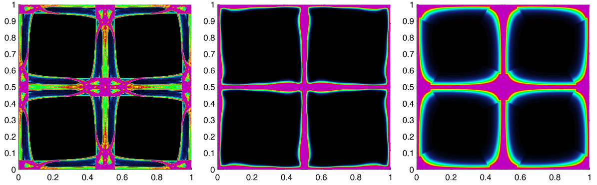
Figure 10: Taylor Green Vortices for St=5St_c : number density field at time t=4 for the Lagrangian tracking (left), for the Eulerian Isotropic Gaussian closure (center), and for the Eulerian Anisotropic Gaussian closure (right).
