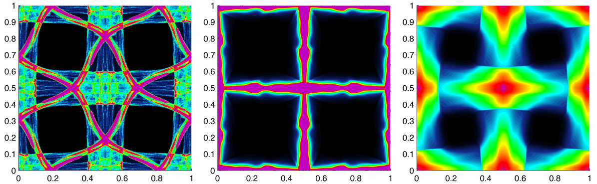
Figure 11: Taylor Green Vortices for St=10St_c : number density field at time t=4 for the Lagrangian tracking (left), for the Eulerian Isotropic Gaussian closure (center), and for the Eulerian Anisotropic Gaussian closure (right).
