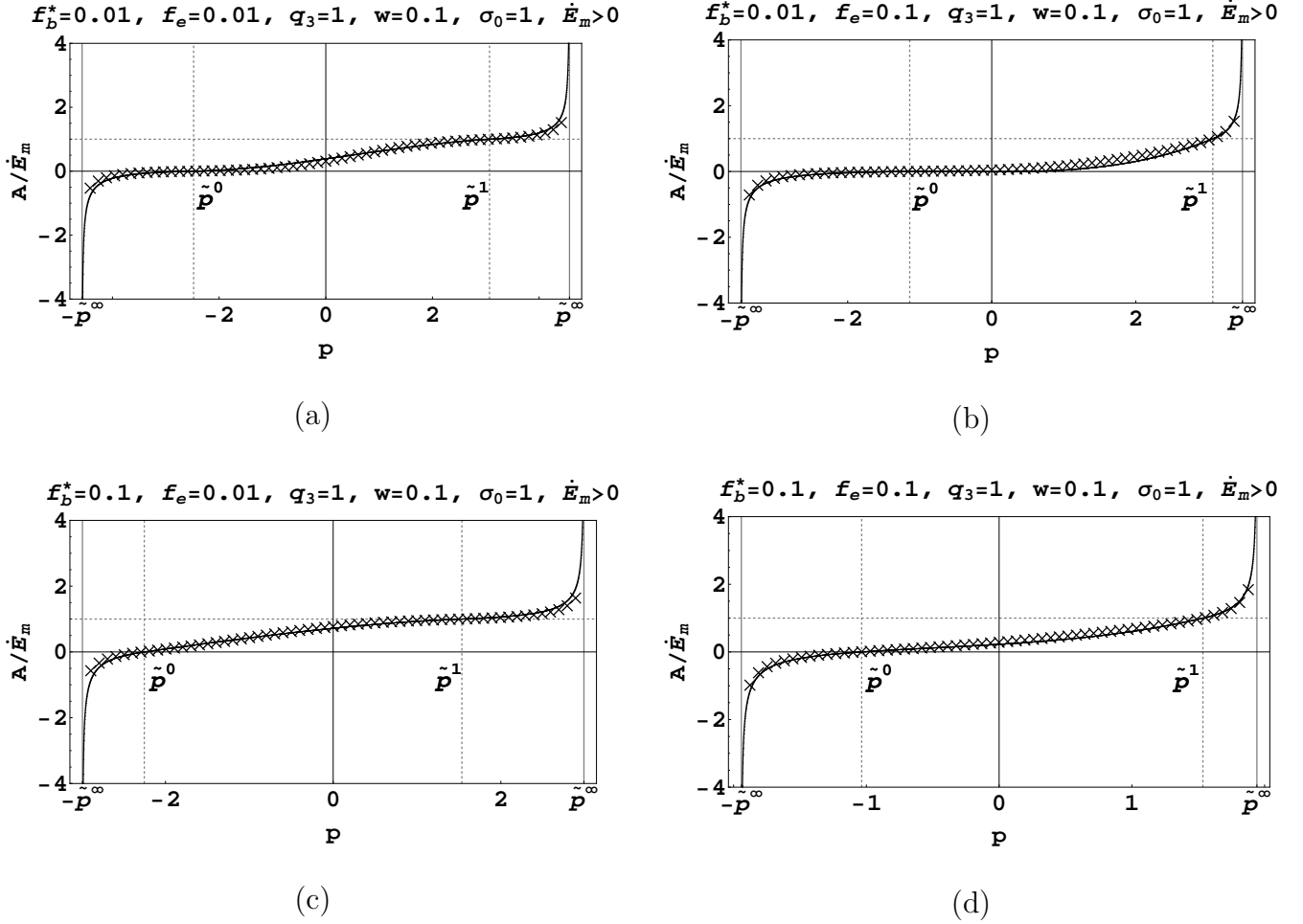
Figure 11: Ellipsoidal intergranular voids. Purely hydrostatic overall strain-rate \dot{E}_{eq} = 0, \dot{E}_m > 0 . Comparison between the exact minimizer A_{sol} for \Phi^+ (crosses) and the approximation \tilde{A} (47) (solid line).
