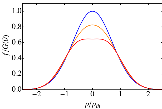
FIG. 2: Color online. Deformation of the momentum distribution of a unitary Bose gas due to three-body losses. From top to bottom: n\lambda_{\text{th}}^3(1 - e^{-4\eta}) = 0 (Blue, Boltzmann gas); n\lambda_{\text{th}}^3(1 - e^{-4\eta}) = 0.05 (Orange) and n\lambda_{\text{th}}^3(1 - e^{-4\eta}) = 0.1 (Red).
