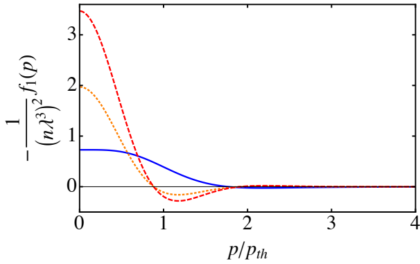
FIG. 3: Correction to the Boltzmann gas: three-body losses vs interactions. The correction to Boltzmann's distribution is plotted for maximal three-body losses ( \eta = \infty , red dashed line), \eta = 0.2 , corresponding to {}^7\text{Li} (Orange dotted line). The blue solid line corresponds to the correction Eq. (21) due to Bose statistics and two-body interactions.
