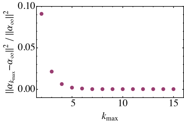
FIG. 1: Convergence of the numerical solution of Eq. (18). We estimate the error on the solution using the norme \|\alpha\|^2 = \langle \alpha | \alpha \rangle and we compare the solution of Eq. (18) obtained by truncation at k = k_{\max} with the “true” result corresponding to k_{\max} = 15 .
