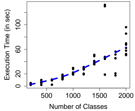
Figure 5: Bootstrap Execution Time
