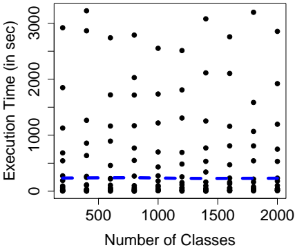
Figure 4: Double Sampling Execution Time
