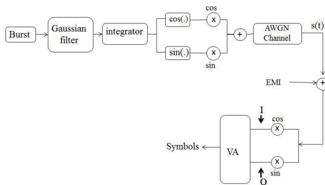
Figure 2: Communication chain (quadratic representation).
