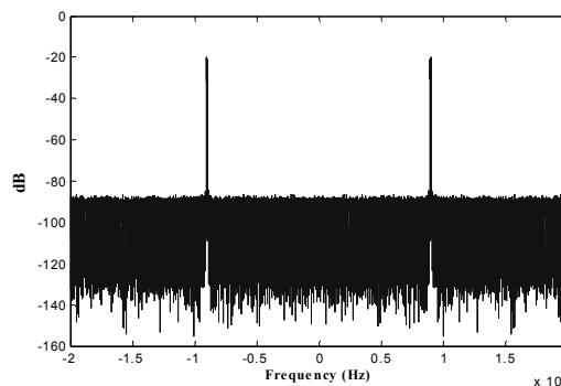
Figure 3: DSP representation of transmitted signal (perfect mode).
