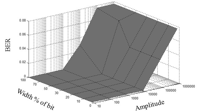
Figure 5: BER in terms of percentage of the disturbance bandwidth and amplitude
