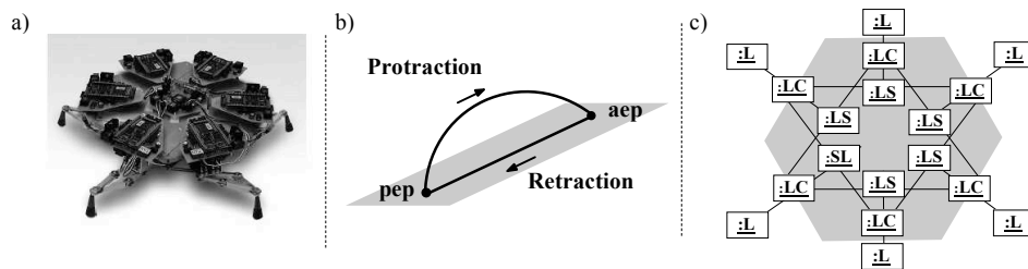
Figure 2. a) Mobile platform, b) Walking cycle, c) Control architecture
