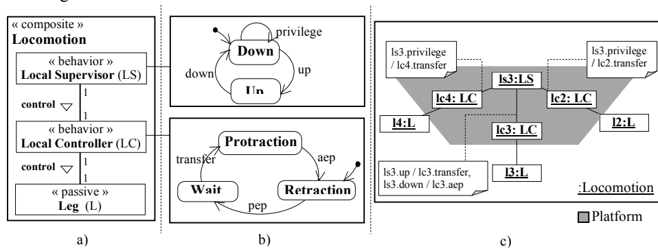
Figure 3: Specification model of the Locomotion function: a) structural aspects, b) behavioral aspects, c) configuration aspects
