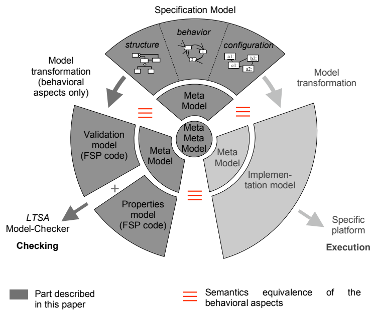
Figure 1. Projection of the behavioral aspects into a process algebra technical space
