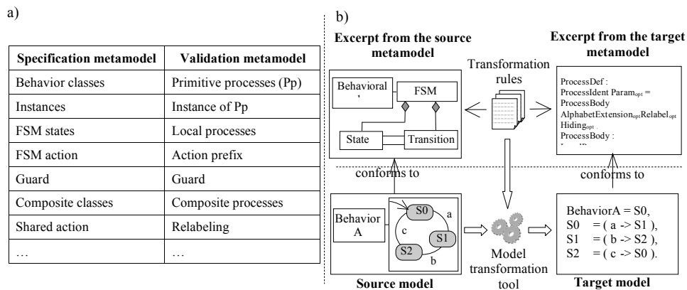
Figure 6.a). Correspondence between the specification and validation metamodel, b) Conceptual representation of metamodeling
