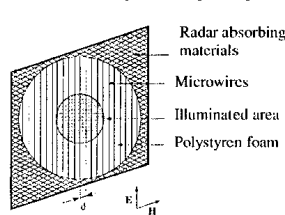
Figure 1 : wire medium and polarization of interest.
