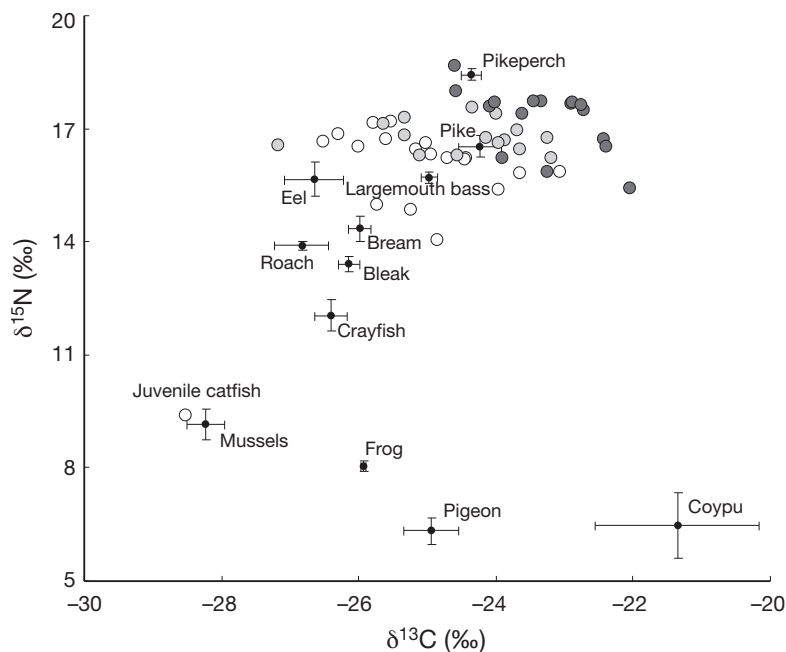
Fig. 3. \delta^{13}\text{C} and \delta^{15}\text{N} biplot of the Tarn River food web. Mean values ( \pm\text{SE} ) are given for all other species except European catfish Silurus glanis , for which individual values are given. Open symbols: small-bodied individuals; closed light grey symbols: medium-bodied individuals; closed dark grey symbols: large-bodied individuals. A single analysed juvenile catfish (60 mm) is also separately indicated
