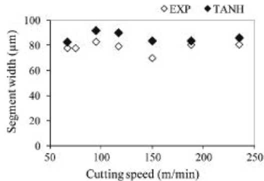
FIGURE 5 Comparison between the segment average width of experimental (EXP) and predicted (TANH) chips for different cutting speeds.
