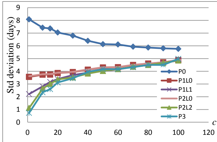
Fig. 6. Waiting time variation vs. unused time slot cost c
