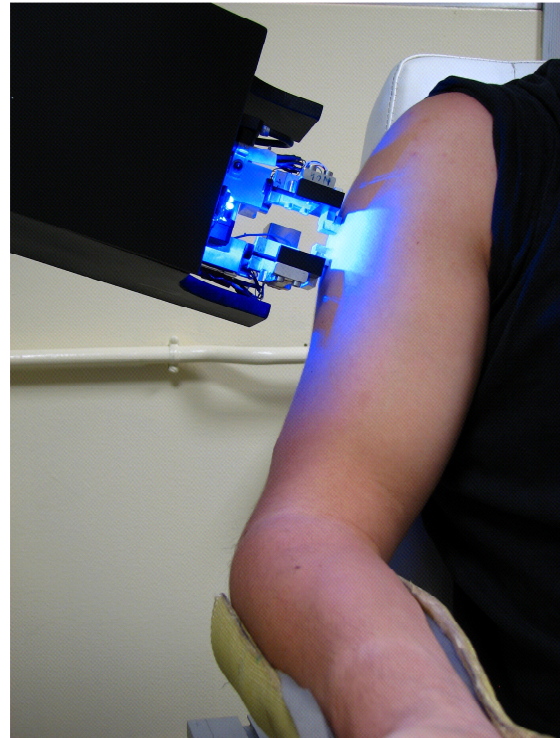
Figure 2. Whole system mounted on a movable frame (left). Measuring head can be rotated to fit with human body necessities, as shown on the right ( in vivo test on the arm ).
