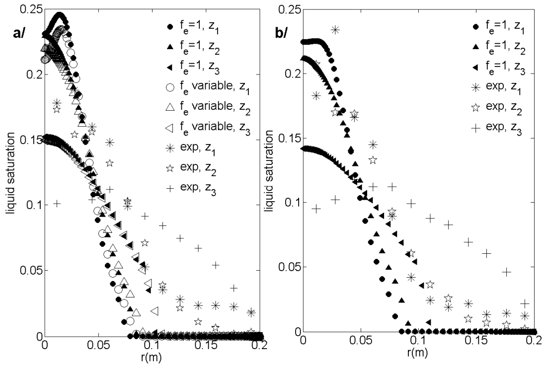
Figure 7: Radial profiles of liquid saturation \theta_L from simulations and experiences for q_L = 16 \text{ m}^3/\text{m}^2\text{h} . F_s = 0.74 \text{ Pa}^{0.5} for the experiments and: a/ F_s = 1.16 \text{ Pa}^{0.5} (cases a and b of Table 1), b/ F_s = 2.21 \text{ Pa}^{0.5} , (case d of Table 1).
