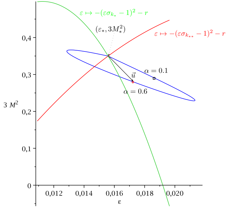
FIGURE 3. Phase diagramm for k_* = 3 , k_{**} = 2 (thus x = 9/4 ) and M_*^2 = 0.4(C + D)_0(x) + 0.6J_2(x) . See Remark 4.1.
