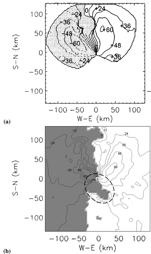
Fig. 6. (a) Observed Doppler velocity values ( \text{m s}^{-1} ) at 0.5^\circ elevation at 14:22 UTC on 22 January 2002; (b) Doppler velocity values ( \text{m s}^{-1} ) deduced from the “Island” experiment at 17:30 at 1000 m altitude. Symbol “R” indicates the location of the Doppler radar, the dashed line contour indicates the location of Réunion island, negative values (away from the radar) are shaded.
