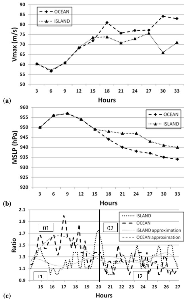
Fig. 5. (a) Time series of the maximum wind velocity ( \text{m s}^{-1} ) at 1000 m altitude for the “Ocean” and “Island” from 3 to 33 h (at 3-h interval); (b) as in (a), except for minimum sea level pressure (MSLP) (hPa); (c) as in (a), except for the ratio between major and minor axes of the eye from 14 to 27 h (1 h interval). Grey lines indicate trend of the ratio (polynomial approximation, 6th order).
