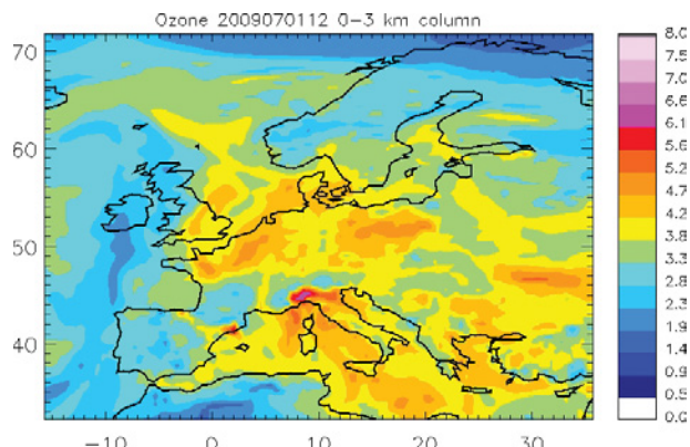
FIG. 2. Map of O_3 partial column (calculated over the height range 0–3 km; height above the model surface) over Europe (x axis: longitude; y axis: latitude) for 1200 UTC (daytime) 1 Jul 2009; units are 10^{17} molecules \text{cm}^{-2} . Red to purple colors denote the relatively high values of the O_3 partial column, indicative of high levels of pollution and a need to monitor AQ; Blue colors denote relatively low values of O_3 partial column. Note the relatively high values over the Po Valley in northern Italy and the Mediterranean and relatively low values over the Alps immediately to the north of the Po Valley. The influence of transport processes on tropospheric O_3 concentrations over southern Europe and the Mediterranean has
